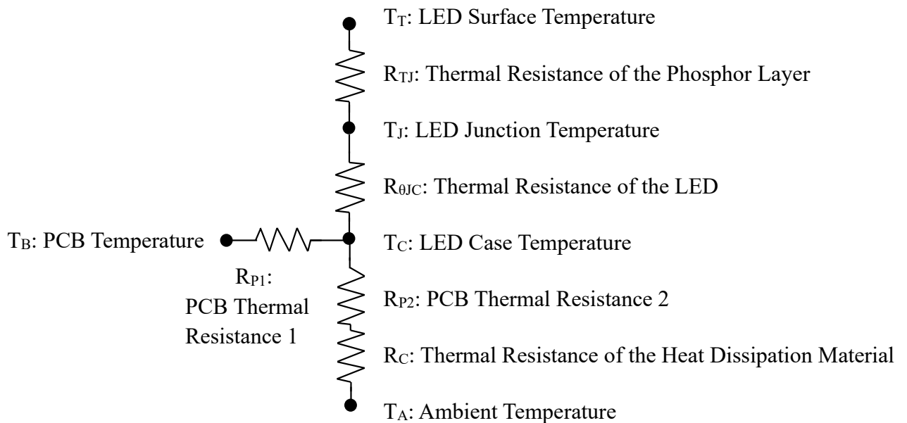
Figure 2. Simplified Thermal Resistance Model
