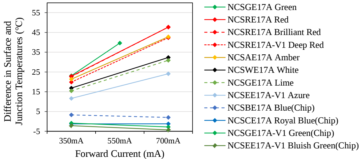
Figure 11. Relationship between the LED Surface and Junction Temperature Differences (For Reference Purposes Only)
