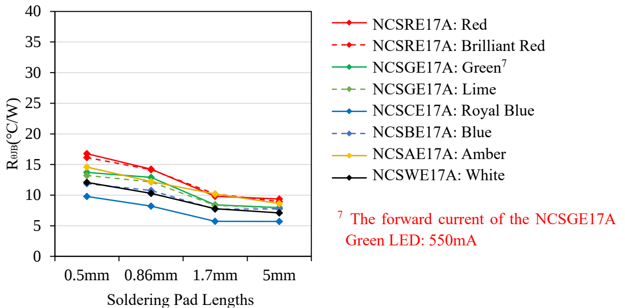
Figure 7. Thermal Resistance ( R_{\theta JB} ) of the evaluated NCSx17 LEDs on Aluminum PCBs (Thermal Conductivity of the Insulating Layer: 5.7\text{W/m}\cdot\text{K} ) at I_F=700\text{mA} 7
