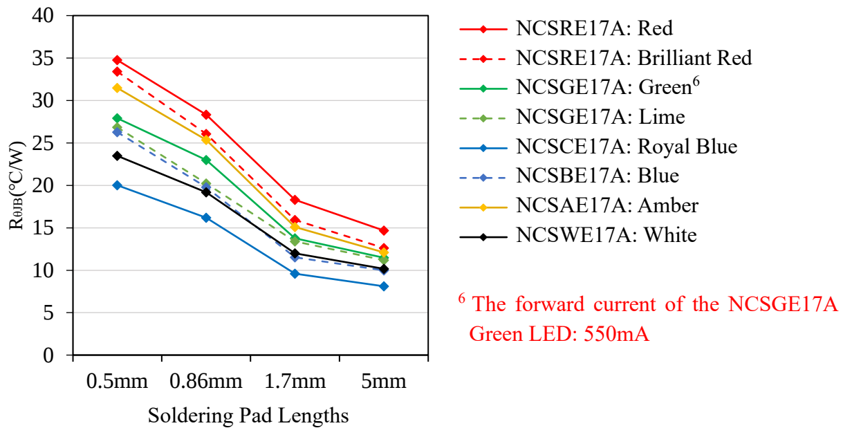
Figure 6. Thermal Resistance ( R_{\theta JB} ) of the evaluated NCSxE17x LEDs on Aluminum PCBs (Thermal Conductivity of the Insulating Layer: 1.8\text{W/m}\cdot\text{K} ) at I_F=700\text{mA} 6
