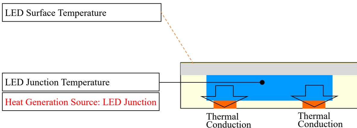
Figure 10. Heat Generation in the LEDs that Do Not Have a Phosphor Layer
