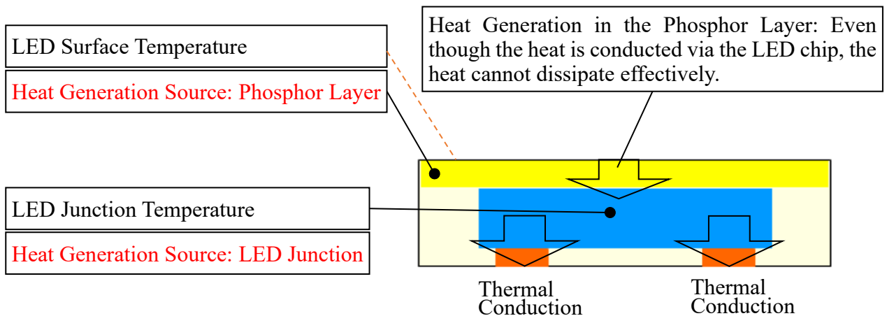
Figure 9. Heat Generation in the LEDs that Have a Phosphor Layer
