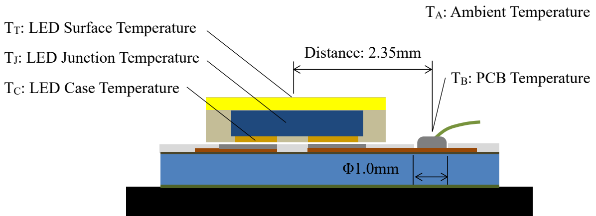
Figure 1. Cross-sectional View of a NCSxE17x LED
